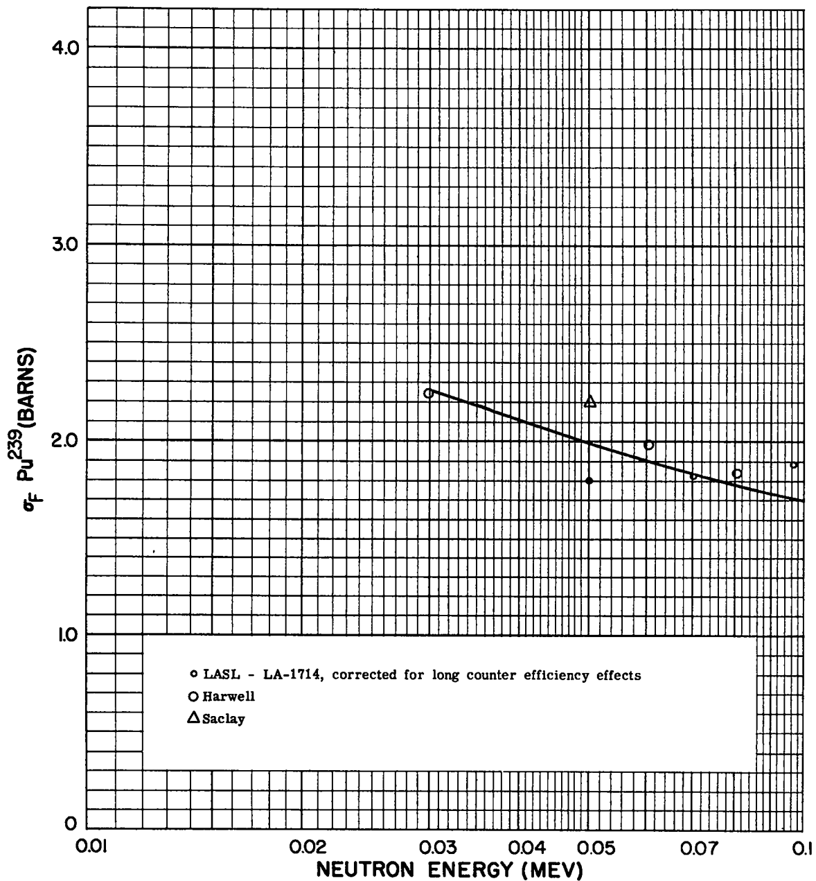
Fig. 4a Fission cross section of \text{Pu}^{239} from 0.01 to 0.1 Mev
