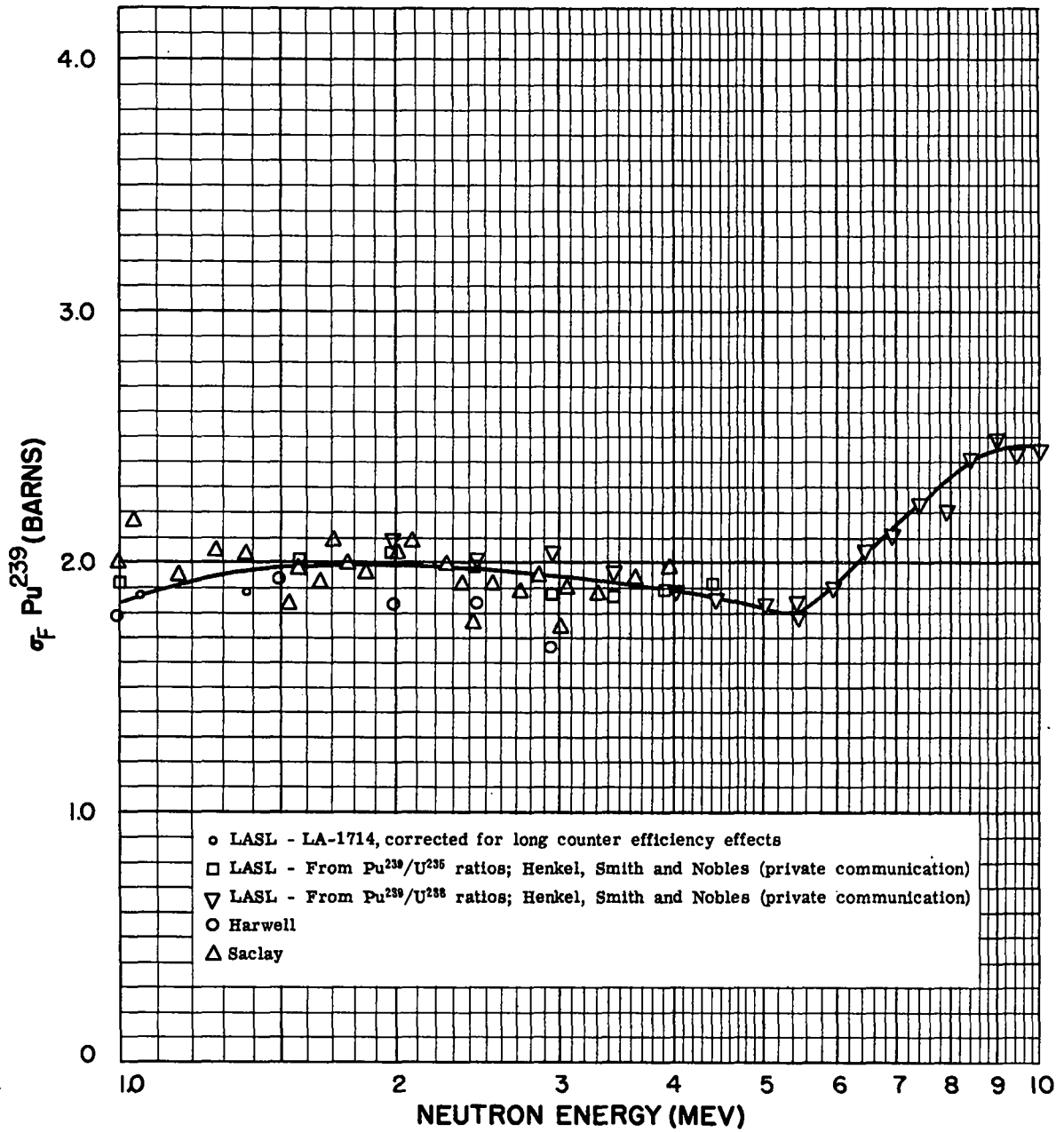
Fig. 4c Fission cross section of \text{Pu}^{239} from 1.0 to 10 Mev
